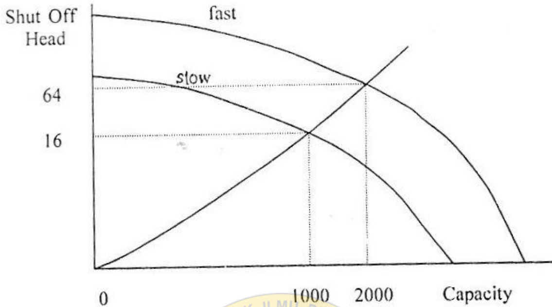
Gambar 5. diagram Kurva H-Q
