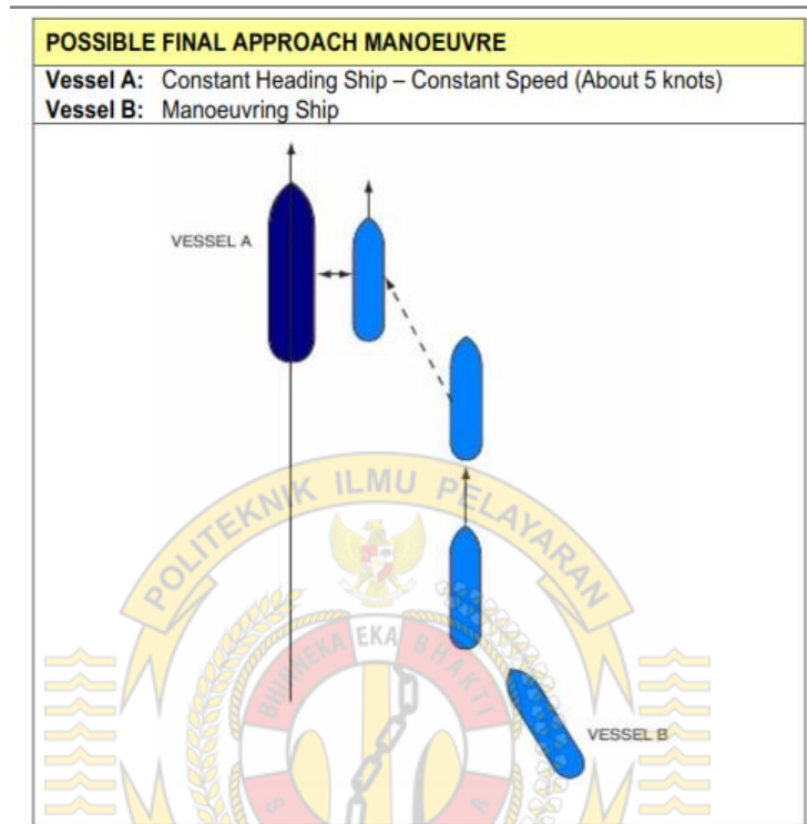
Olah Gerak Kapal Ship to Ship Transfer
