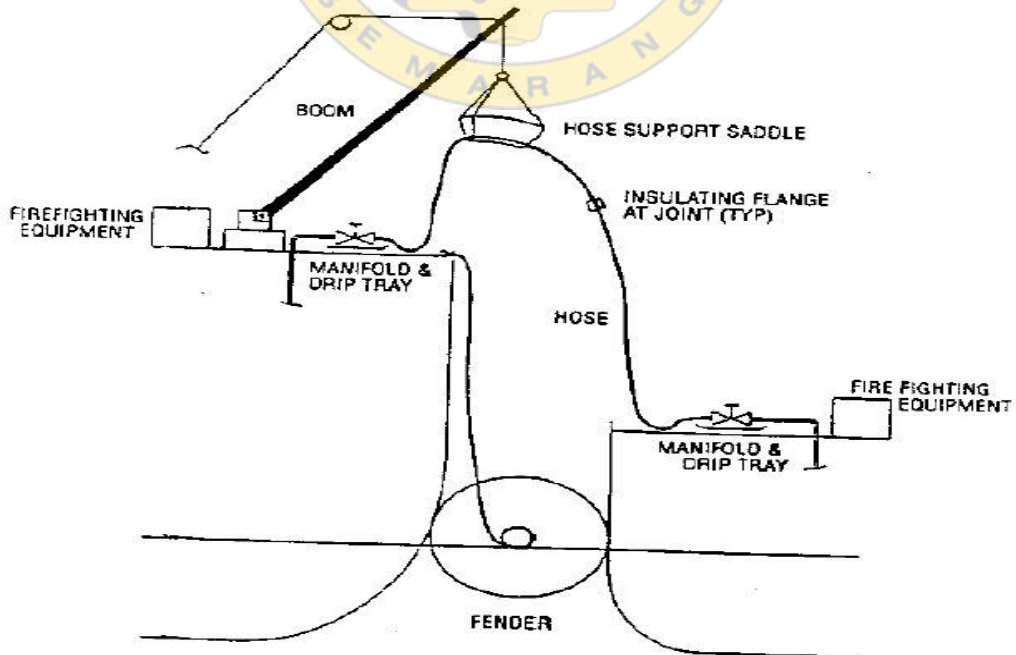
Ship to Ship Transfer Arrangement
