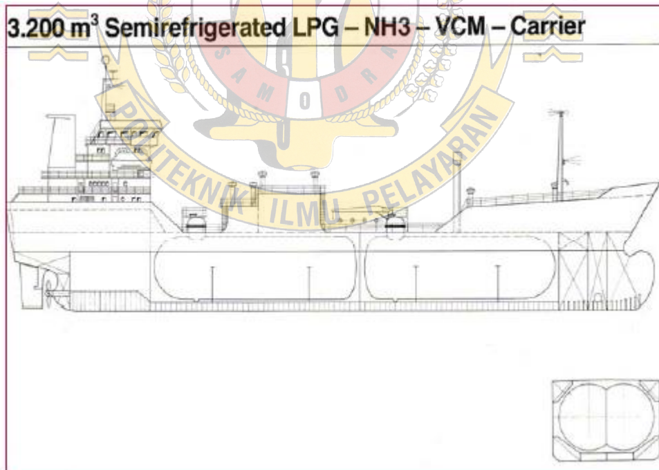
Gambar 5.4 Kapal LPG tipe semi refrigerated
