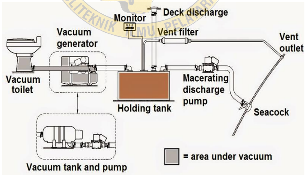
Evac pump vacuum skemati
