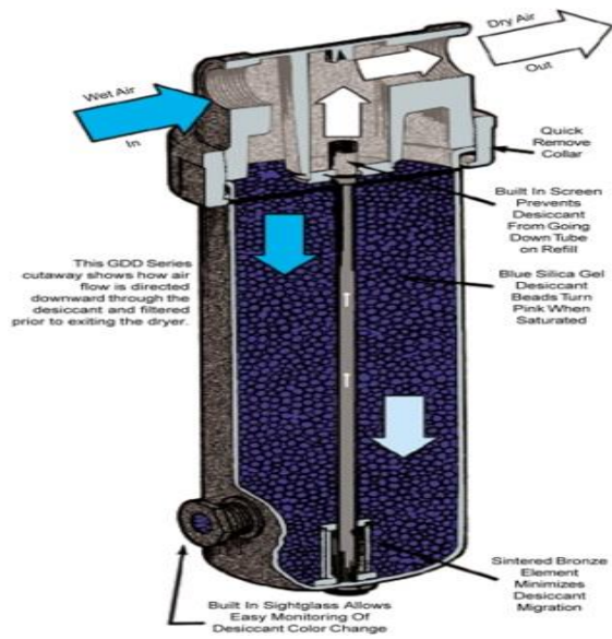
Skema gambar adsorption dryer
